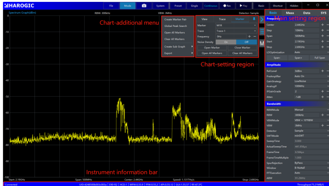
Figure 2 SASudio4 default UI after launching with HAROGIC SAM60 M3.
